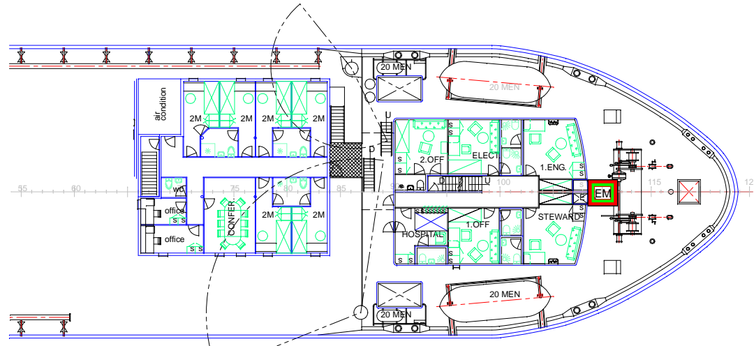
FORCASTLE DECK
