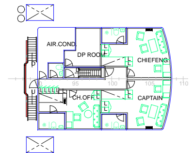
CAPTAIN'S DECK
