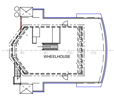
BRIDGE DECK
