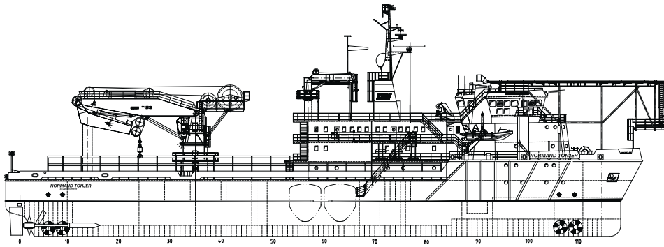
PROFILE VIEW
