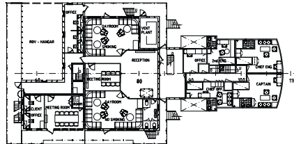
CAPTAINS DECK
