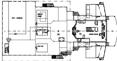
BRIDGE DECK
