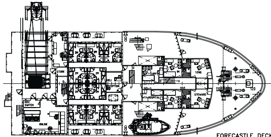
FORECASTLE DECK
